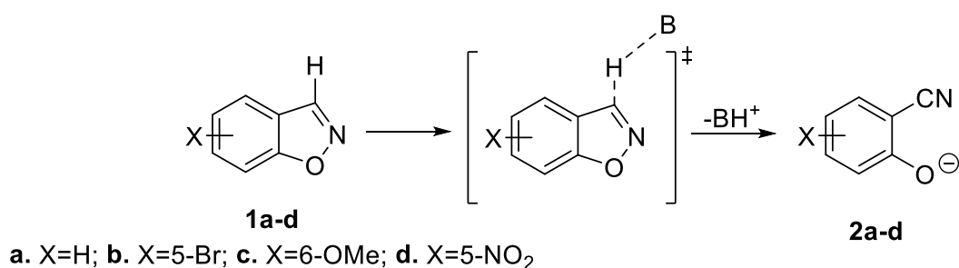
Scheme 1: Kemp elimination.
