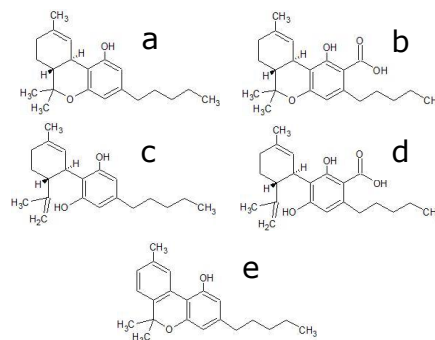
Figure 1. Cannabinoids.
