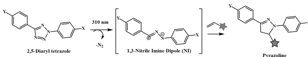
Figure 1. Photogeneration of NI, which can react with an alkene to form a pyrazoline.
